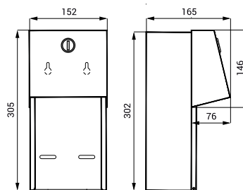
SLZN 26Z 95261 Stainless steel recessed holder of toilet paper
