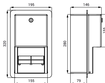
SLZN 37 95370 Stainless steel holder for a big coils of toilet paper
